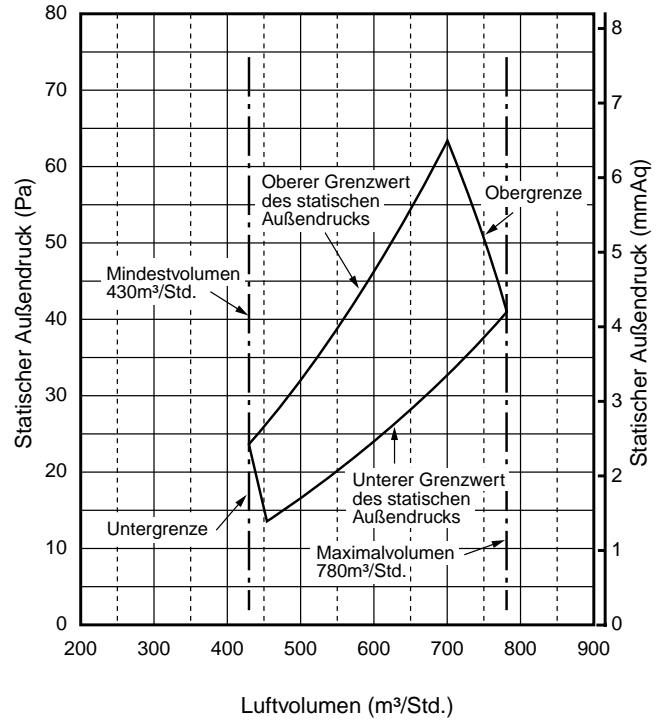
Abb. 3 RAS-M16GDCV-E, RAS-M16GDV-E
